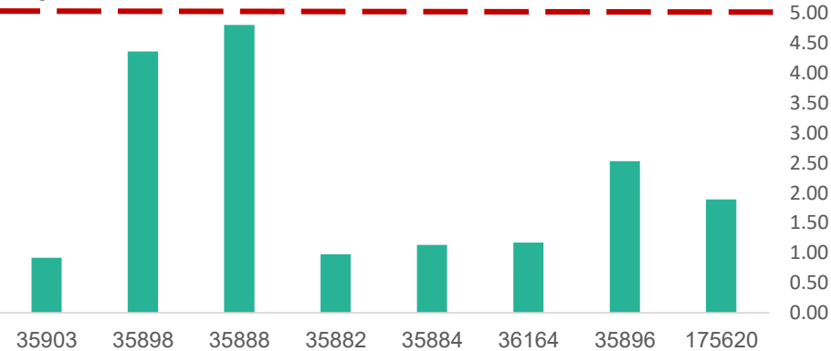
2024 - SO 2 Emission
