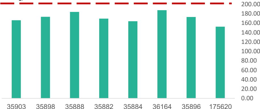
2024 - CO Emission
